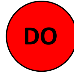
Dissolved Oxygen
